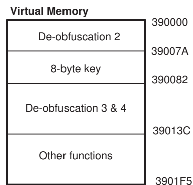
Fig. 3. De-obfuscated code in the virtual memory
