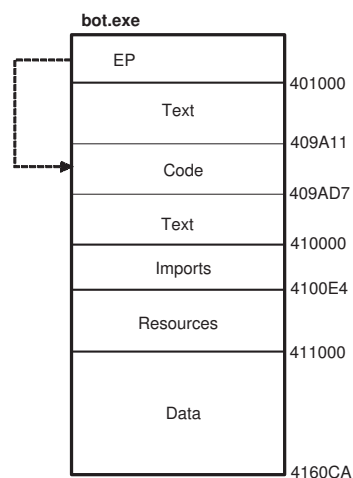
Fig. 2. Segments of the bot.exe binary file
