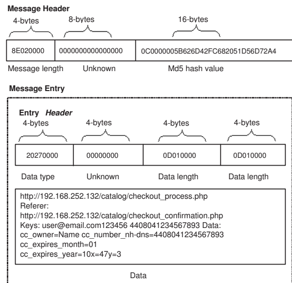
Fig. 7. A decrypted sample message
