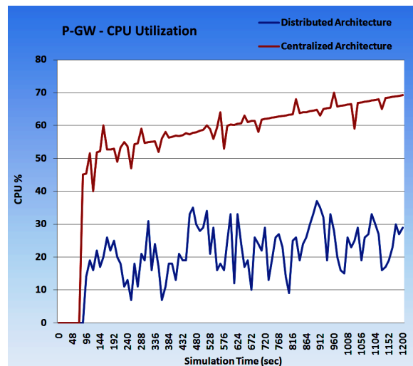
Figure 10. P-GW: CPU Utilization in Both Architectures
