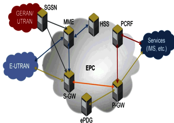
Figure 3. LTE EPC [24]
