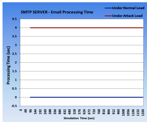
Figure 9. SMTP Server: Email Processing Time/Email in Both Scenarios
